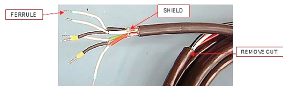
Figure 2: M5000 cables
