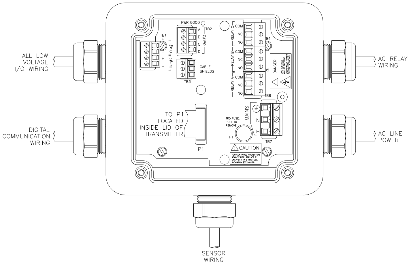
Figure 17 – Q46 Connections
