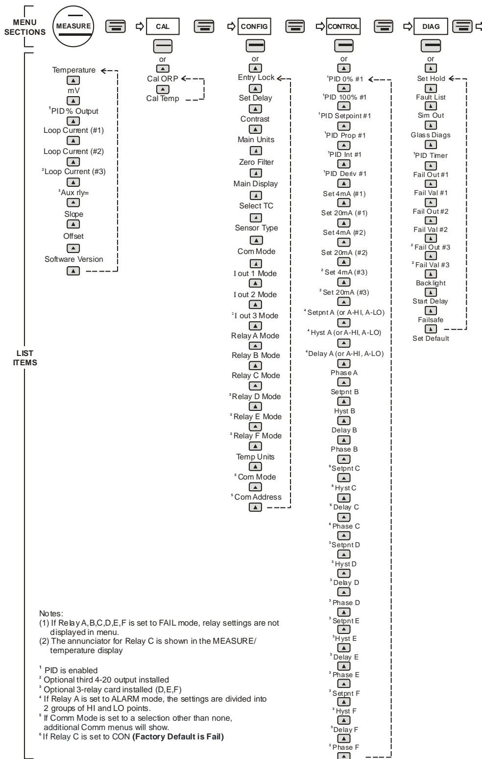
Figure 30 - Software Map
