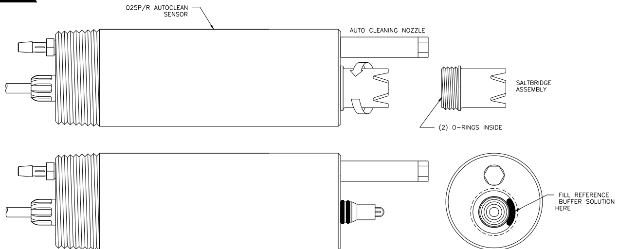
Figure 34 - Replacing the Saltbridge and Reference Buffer
