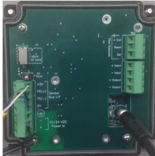
Figure 23 – MetriNet PC Cable Connection
