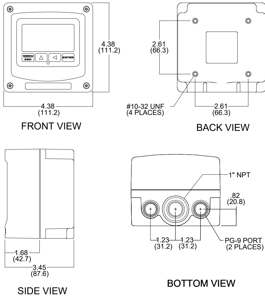
Figure 4 - Enclosure Dimensions
