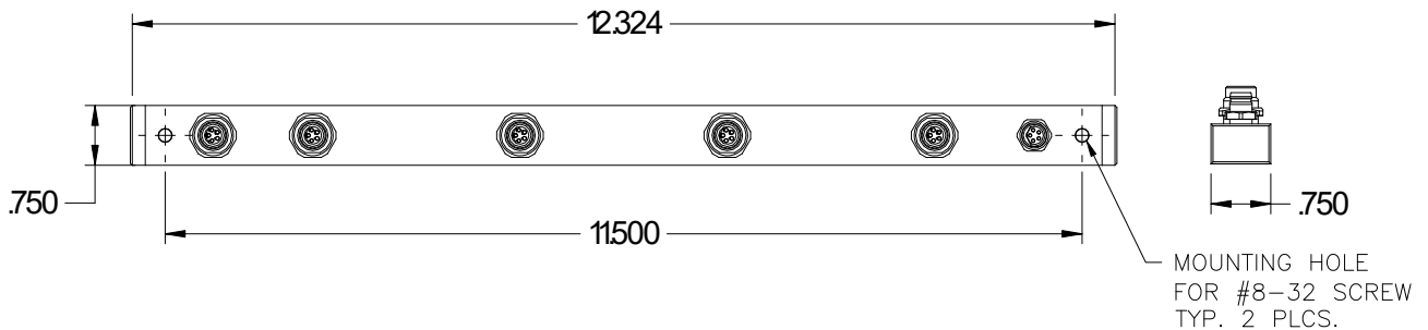
Figure 9 - Sensor Bus Bar Interface
