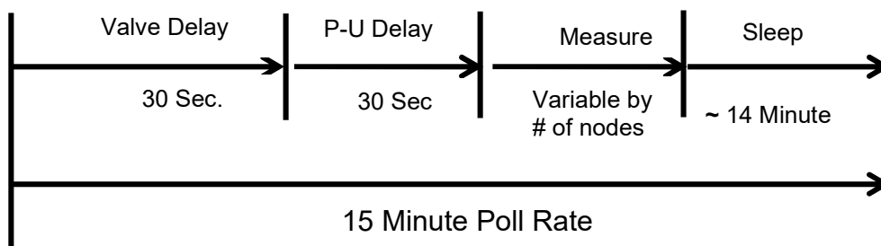
Figure 11 – Cycle Mode Schematic
