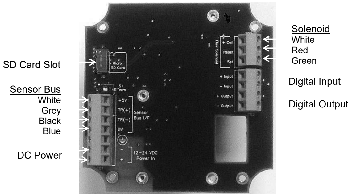
Figure 12 – External Connections
