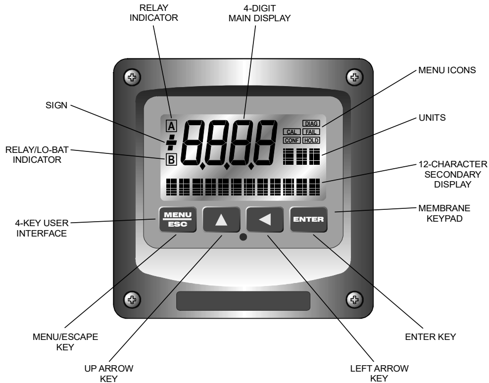
Figure 15 – MetriNet Controller Interface
