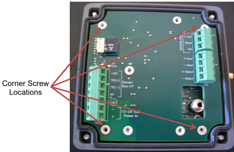
Figure 21 – MetriNet Rear Panel SIM Access
