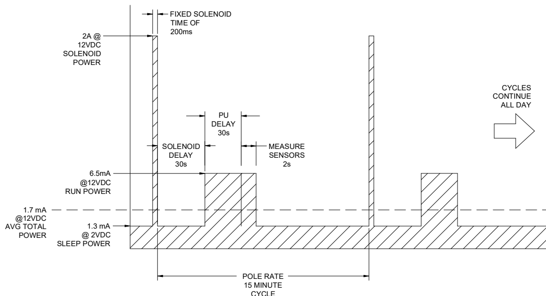
Figure 14 – Average vs Pulse Power, and State Diagram
