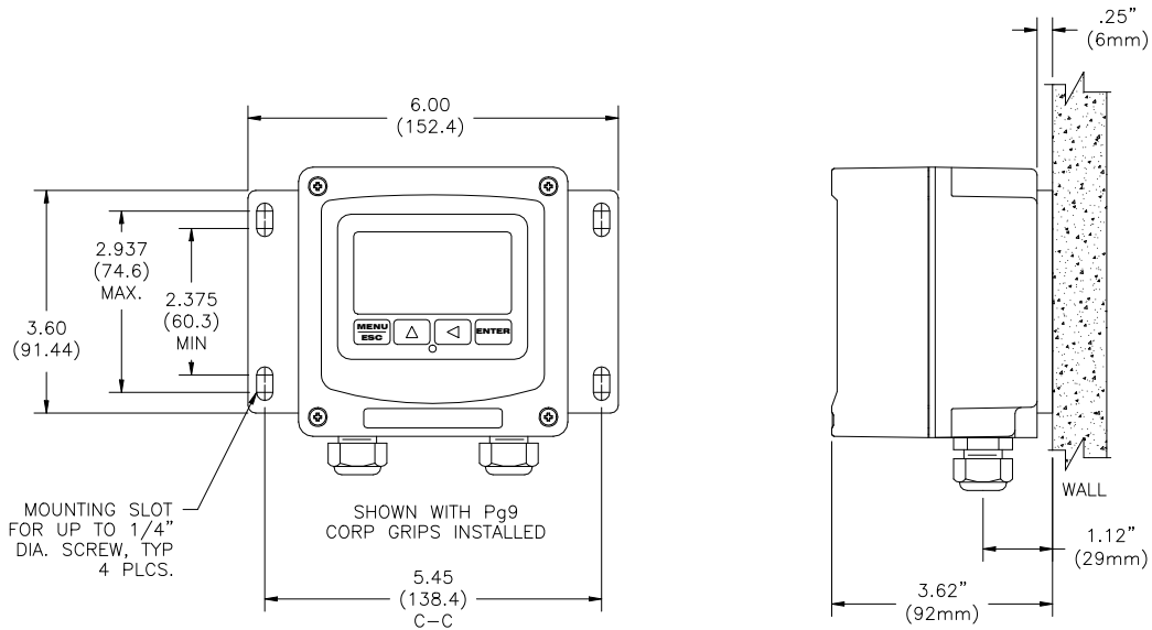
Figure 5 - Wall Mount
