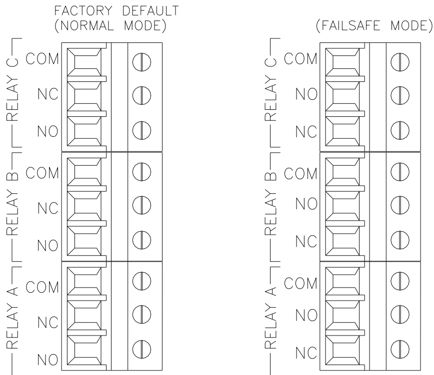
Figure 11 - Relay Contacts
