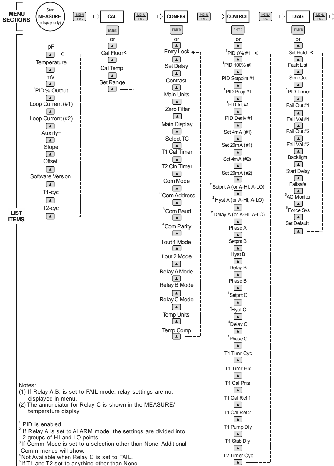
Figure 17 - Software Map
