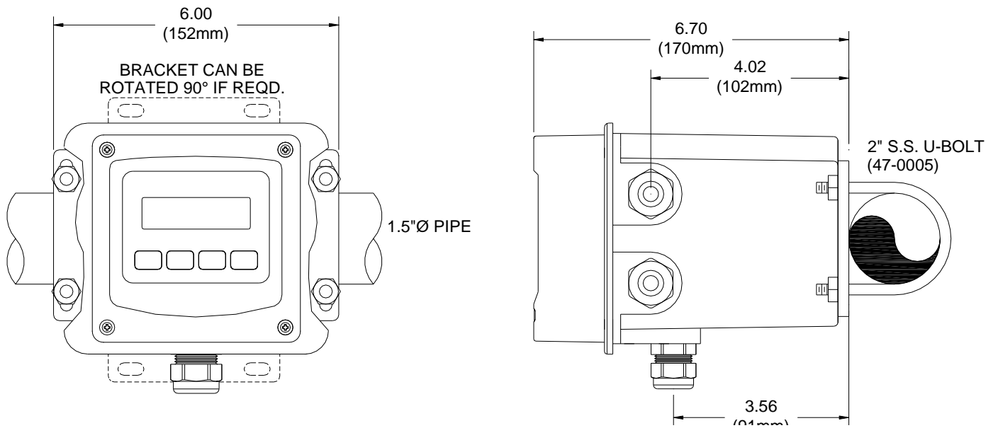
Figure 4 - Pipe Mounting Diagram
