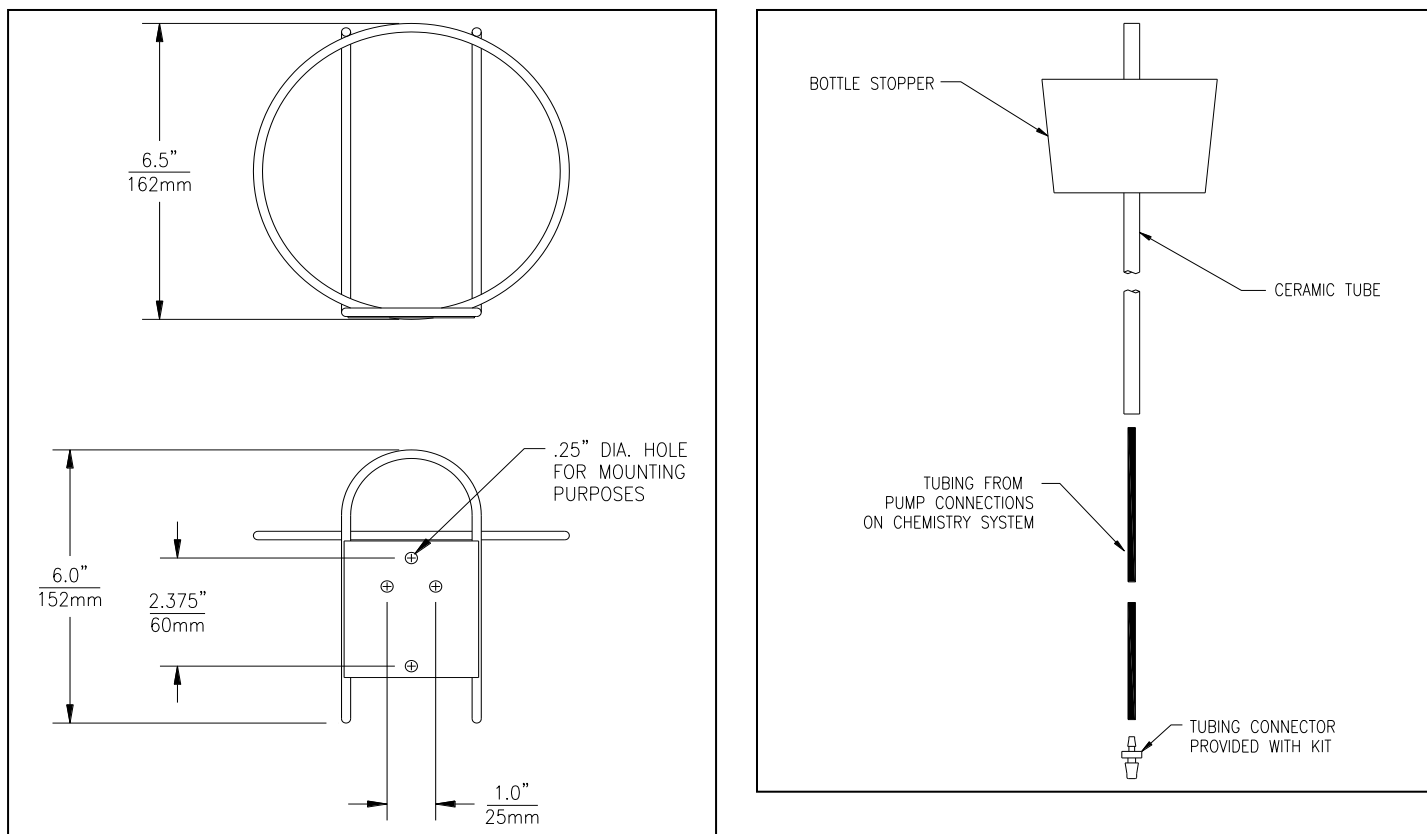
Figure 8 - Bottle Bracket & Reagent Feed Assembly
