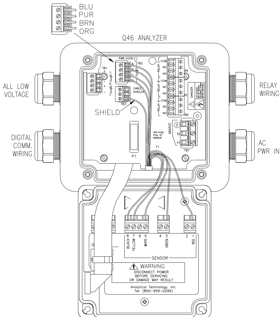
Figure 10 - Sensor and Control Connection
