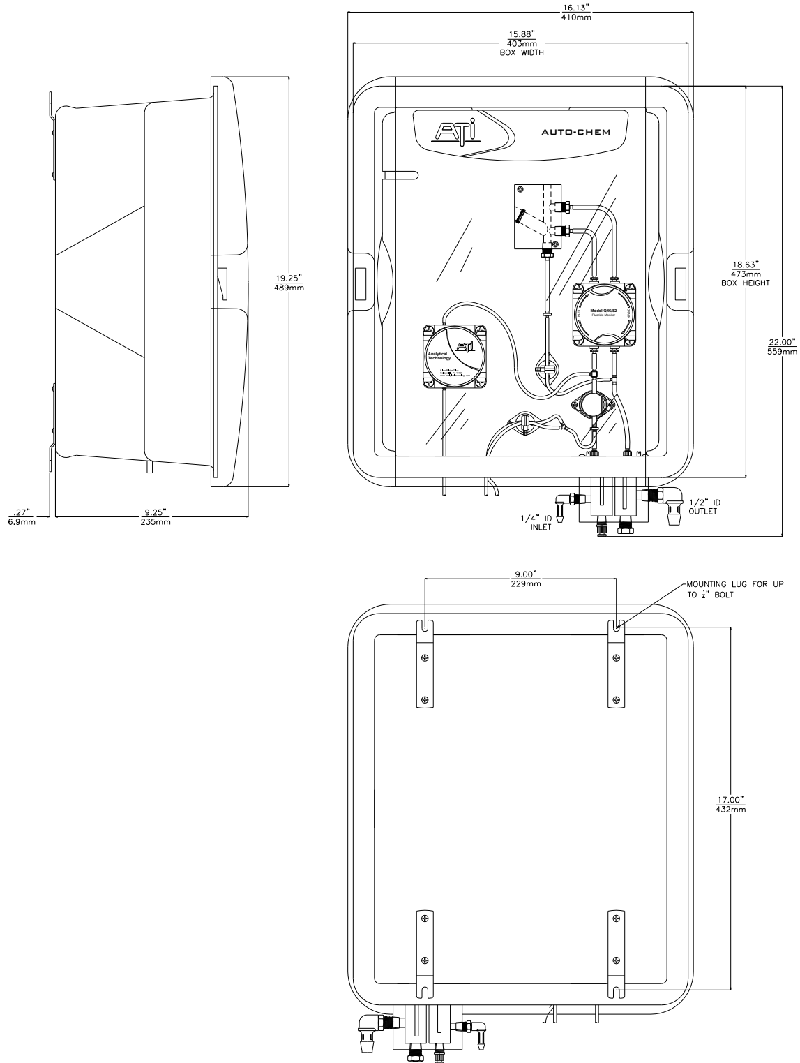
Figure 7 – Auto-Chem Dimensional Drawing
