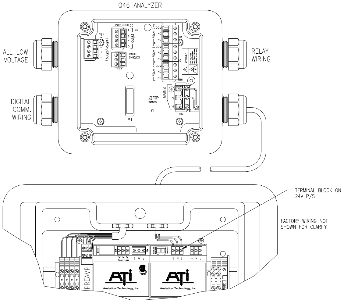
Figure 14 - Analyzer Connection from Autochem
