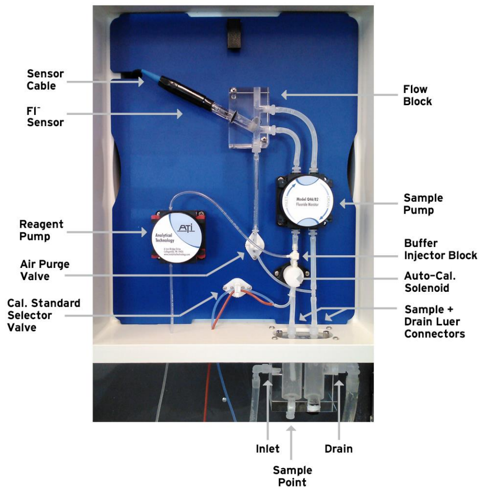
Figure 15 – Auto-Chem Panel Components
