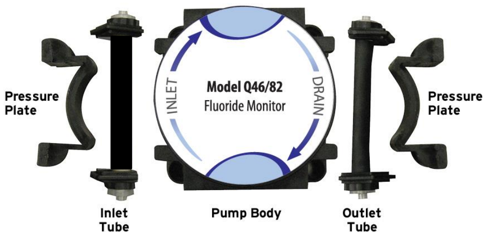
Figure 21 – Sample Pump Exploded View
