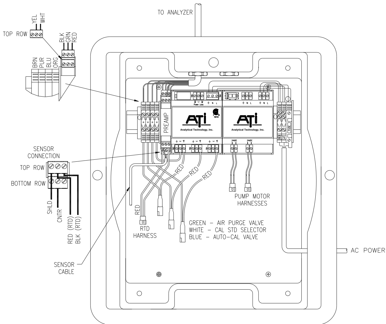
Figure 13 - Auto-Chem Customer Wiring
