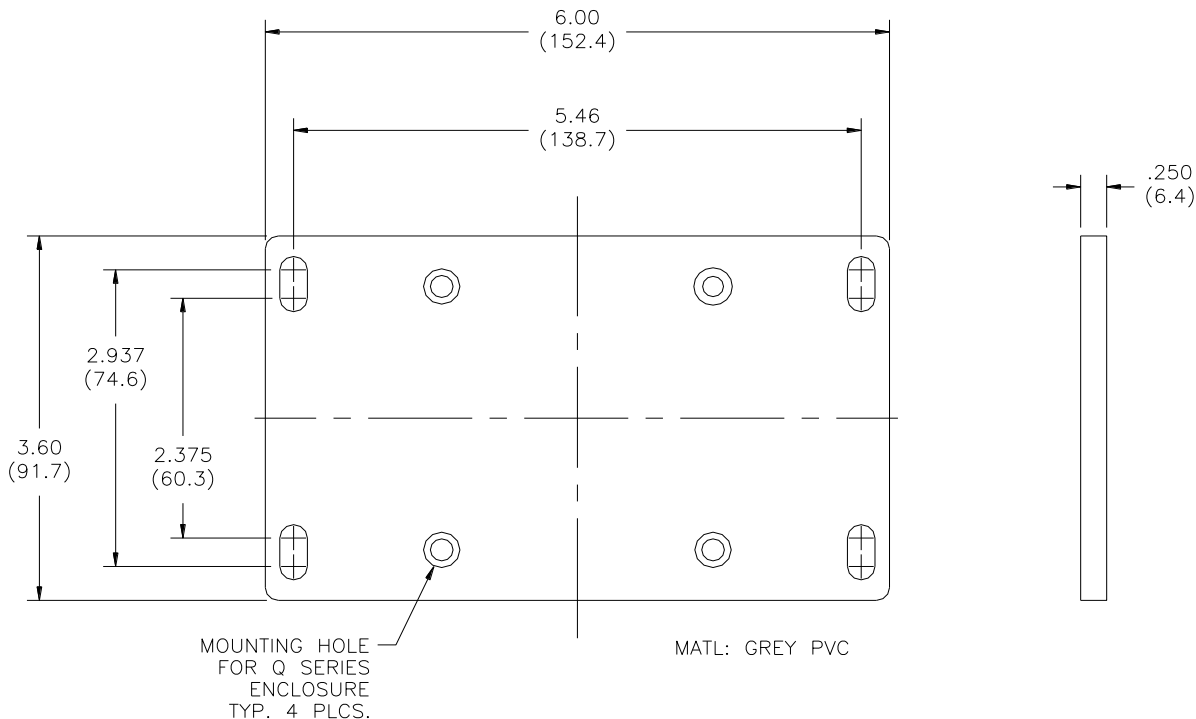
Figure 3- Wall or Pipe Mount Bracket
