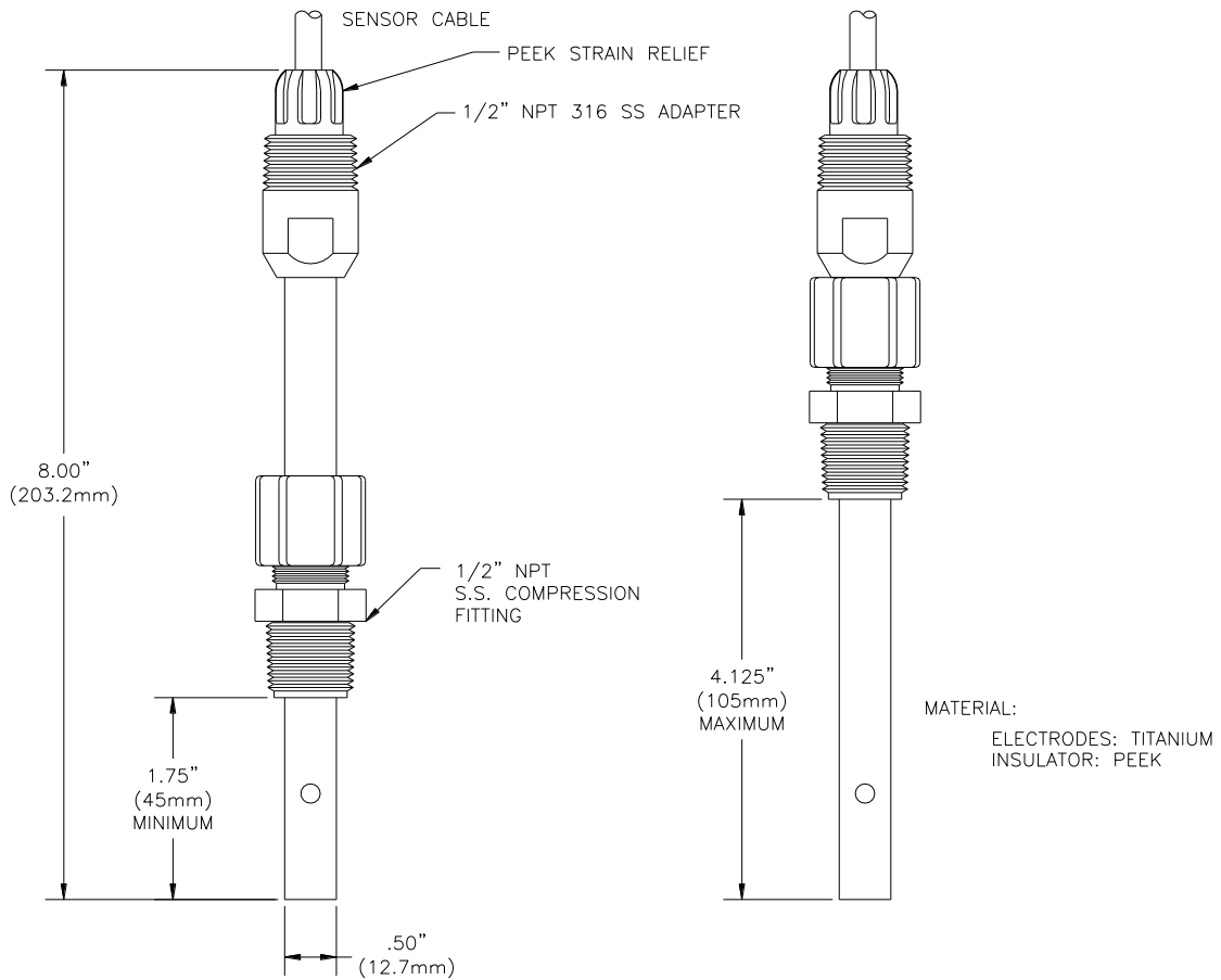
Figure 6 – Insertion/Submersible Style Sensor Dimensions
