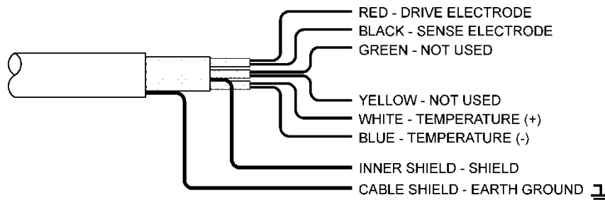
Figure 12 - Cable Description, Model Q25C2
