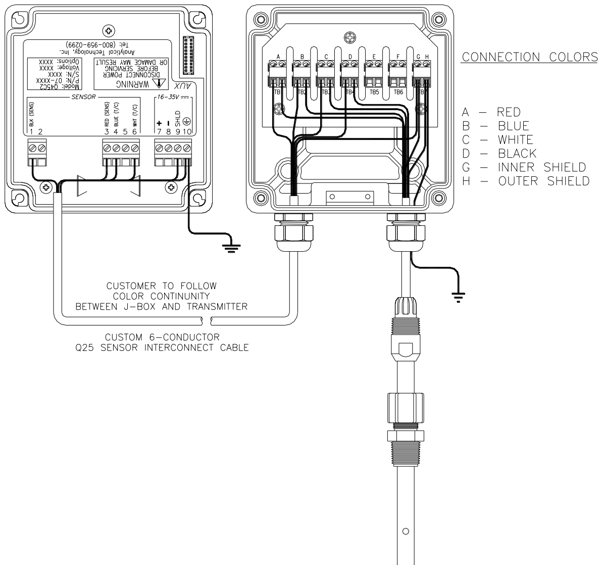
Figure 14 - Junction Box Interconnect Wiring
