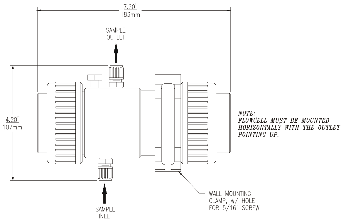
Figure 11 - Flowcell Dimensions
